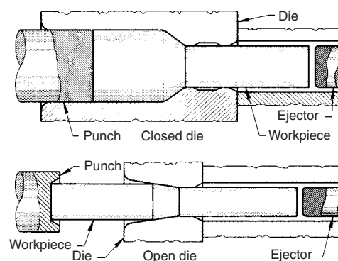
Fig. 12 End of stroke in the forward extrusion of a stepped shaft in a closed die and an open die
