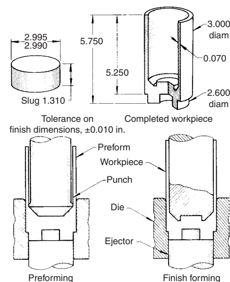
Fig. 19 Aluminum alloy 1100-O housing that was extruded in two operations because of an internal boss. Dimensions given in inches
